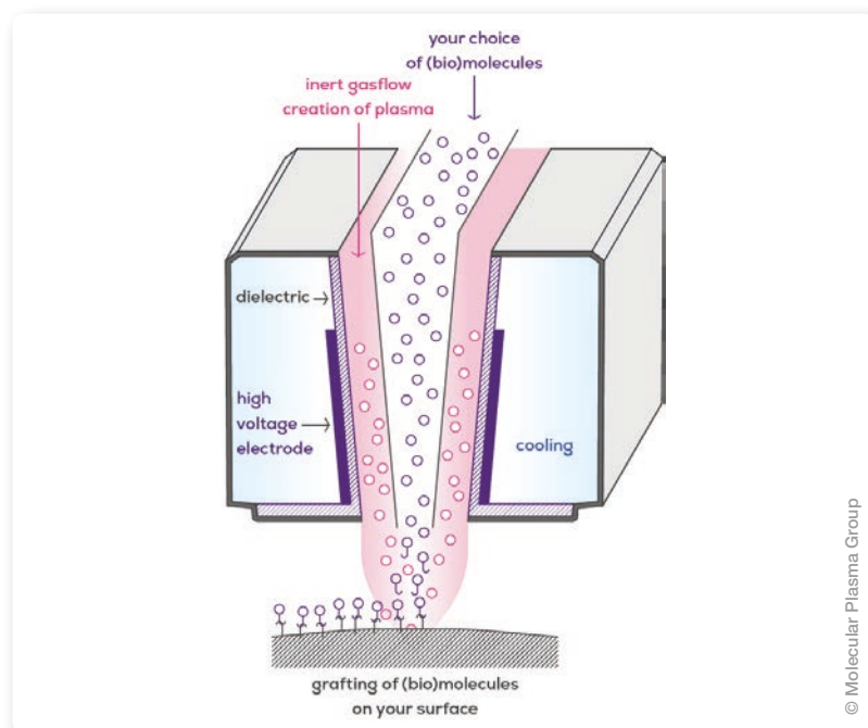
PlasmaLine linear head enables homogeneous plasma coating up to 1.5 m width.
